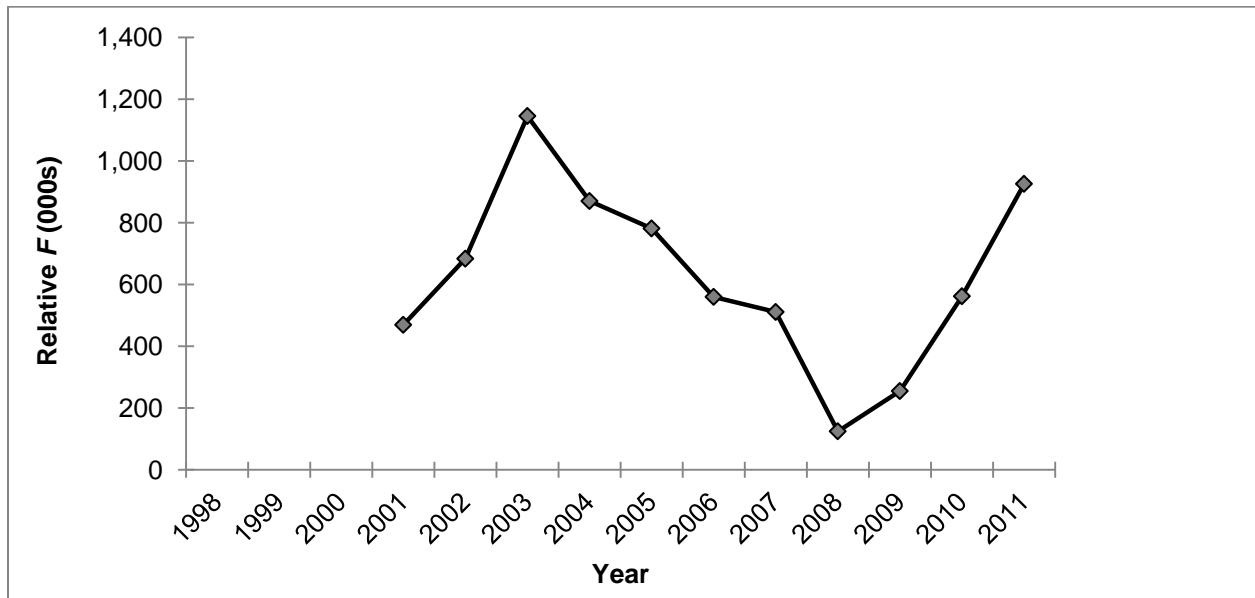
Figure 5. Commercial landings of roes by all gear types (March–May) compared to the female electrofishing index (March–May; top graph) and annual estimates of female relative F based on these data (bottom graph) for Albemarle Sound, 2000–2011. The error bars in the top graph represent \pm 1 standard deviation.
