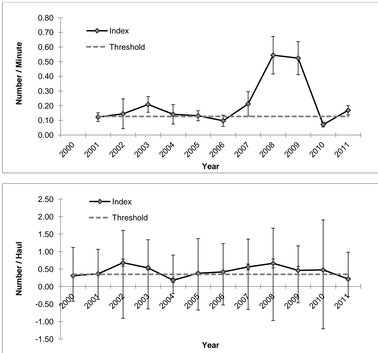
Figure 3. Female index from electrofishing survey (March–May; top graph) and female index from IGNS (January–May; bottom graph) for Albemarle Sound, 2000–2011. The error bars represent \pm 1 standard deviation. Threshold represents 25 th percentile (where 75% of all values are greater).
