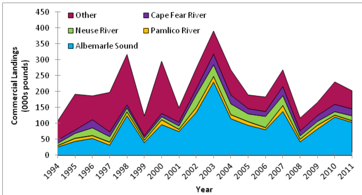
Figure 2. Commercial landings of American shad in North Carolina by water body, 1994–2011.
